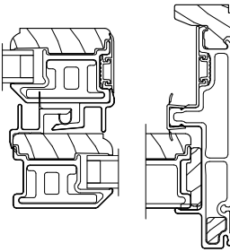
Stile and Jamb Covers Interior Painted Units Only
